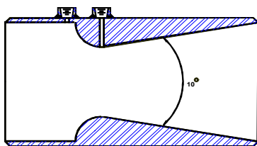
WELD-IN LOW LOSS BAR VENTURI
